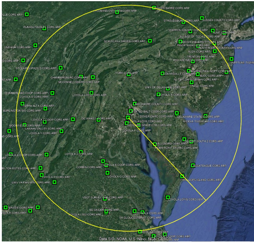
Figure 9-14: Example of CORSs plotted with respect to a 250 km radius from the centroid of the project
